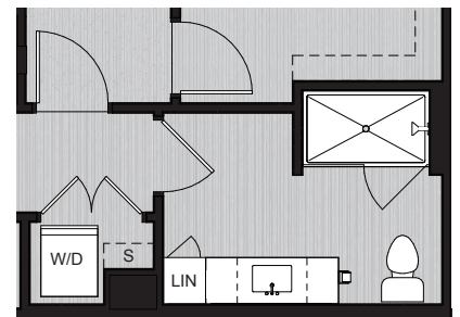
ALTERNATE LAYOUT IN SELECT UNITS
